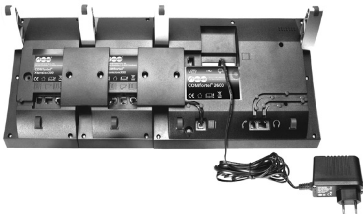
Abb. 6: Assembling and connecting the COMfortel Xtension300 key extension modules
